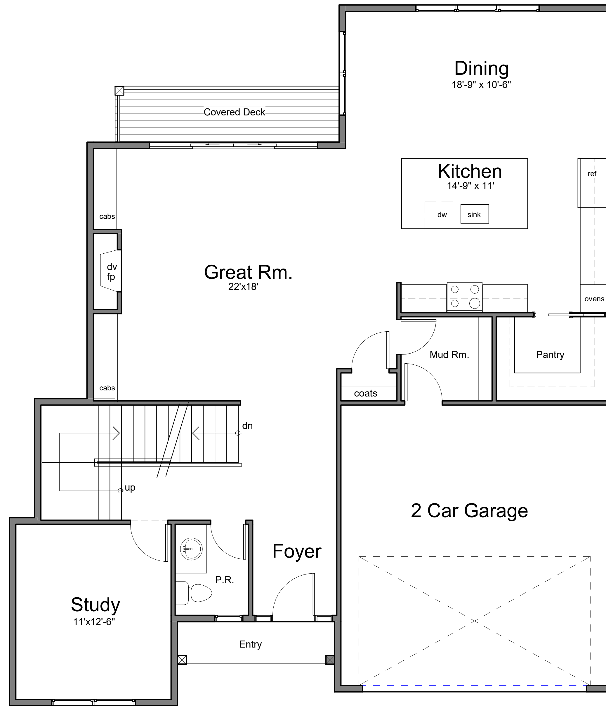
FIRST FLOOR - 9' CEILING HT.
