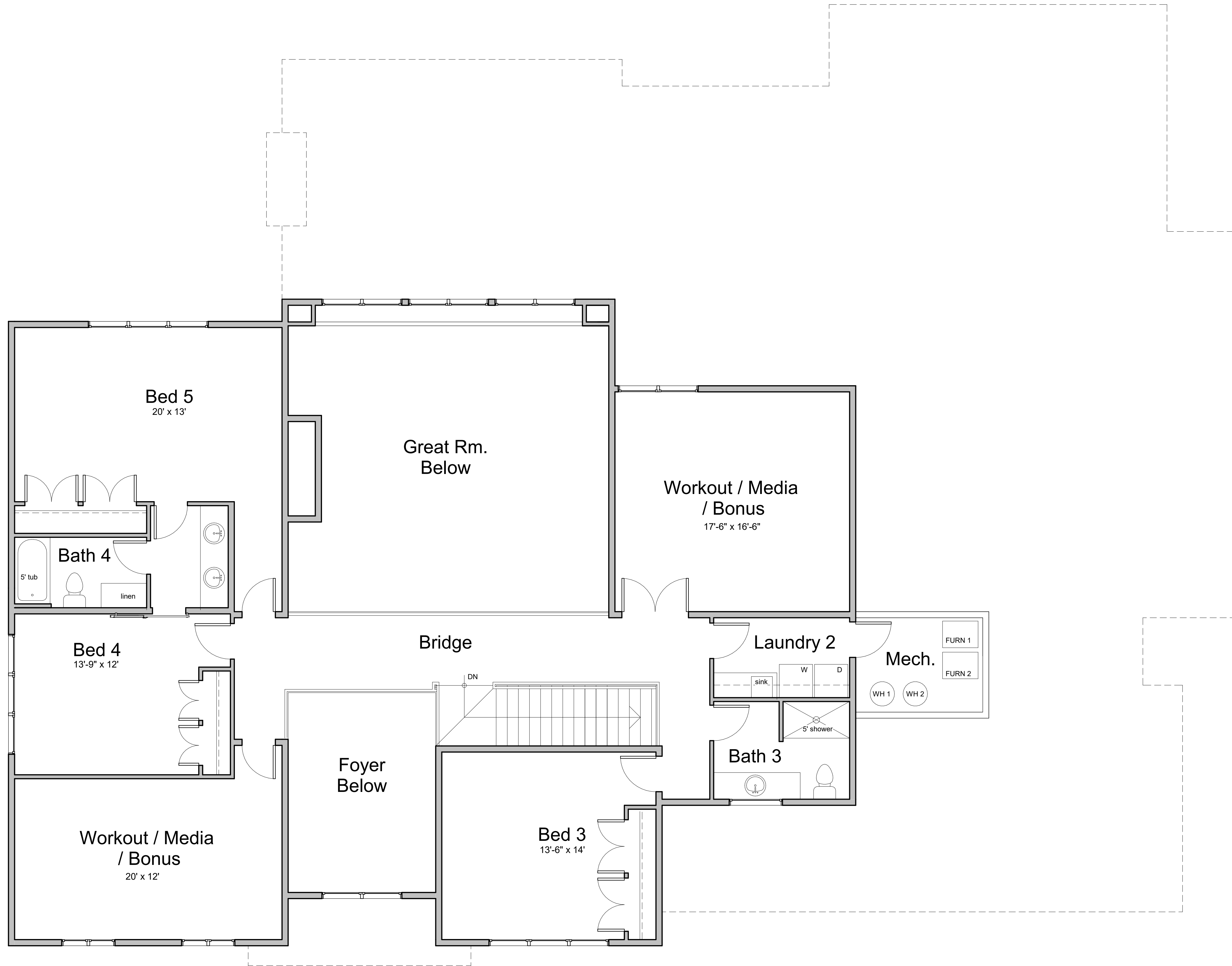
SECOND FLOOR PLAN - 9' CEILING HT.
