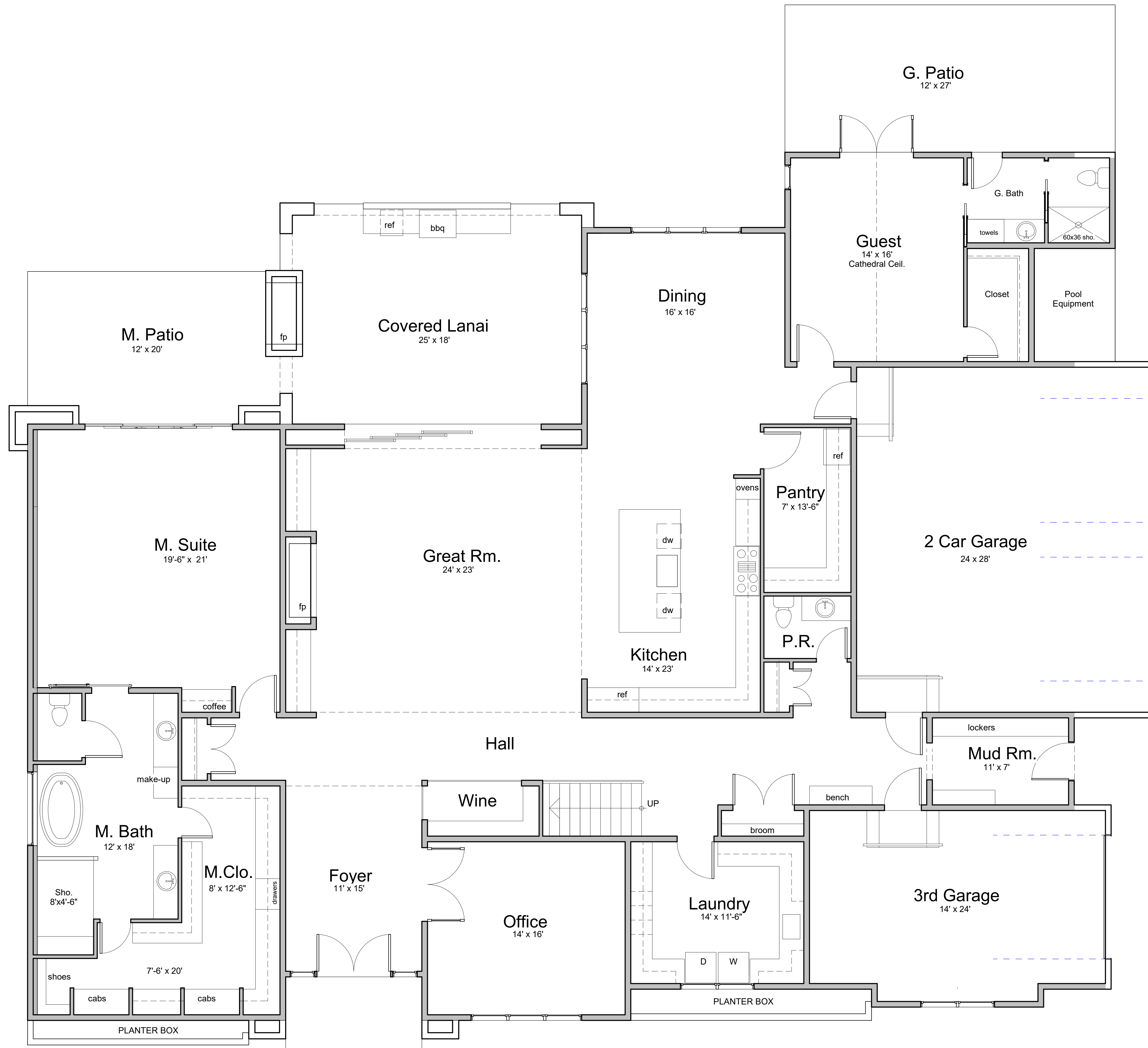
FIRST FLOOR PLAN - 10' CEILING HT.
